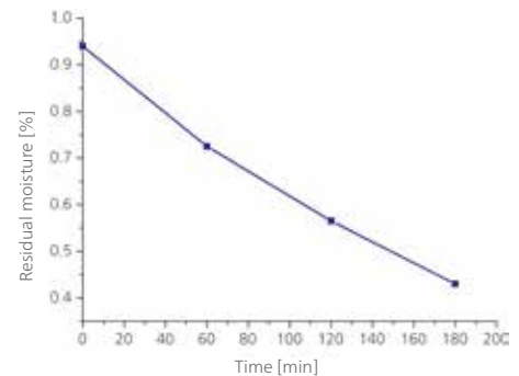
Residual Moisture as a Function of Process Time
